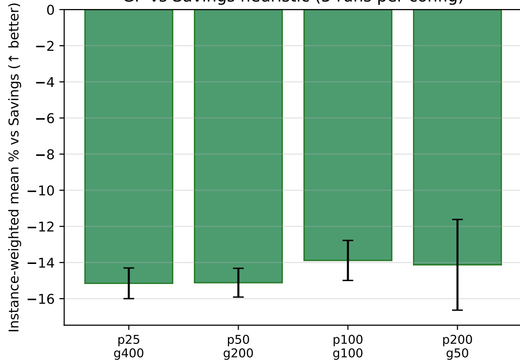
GP vs Savings heuristic (5 runs per config)
