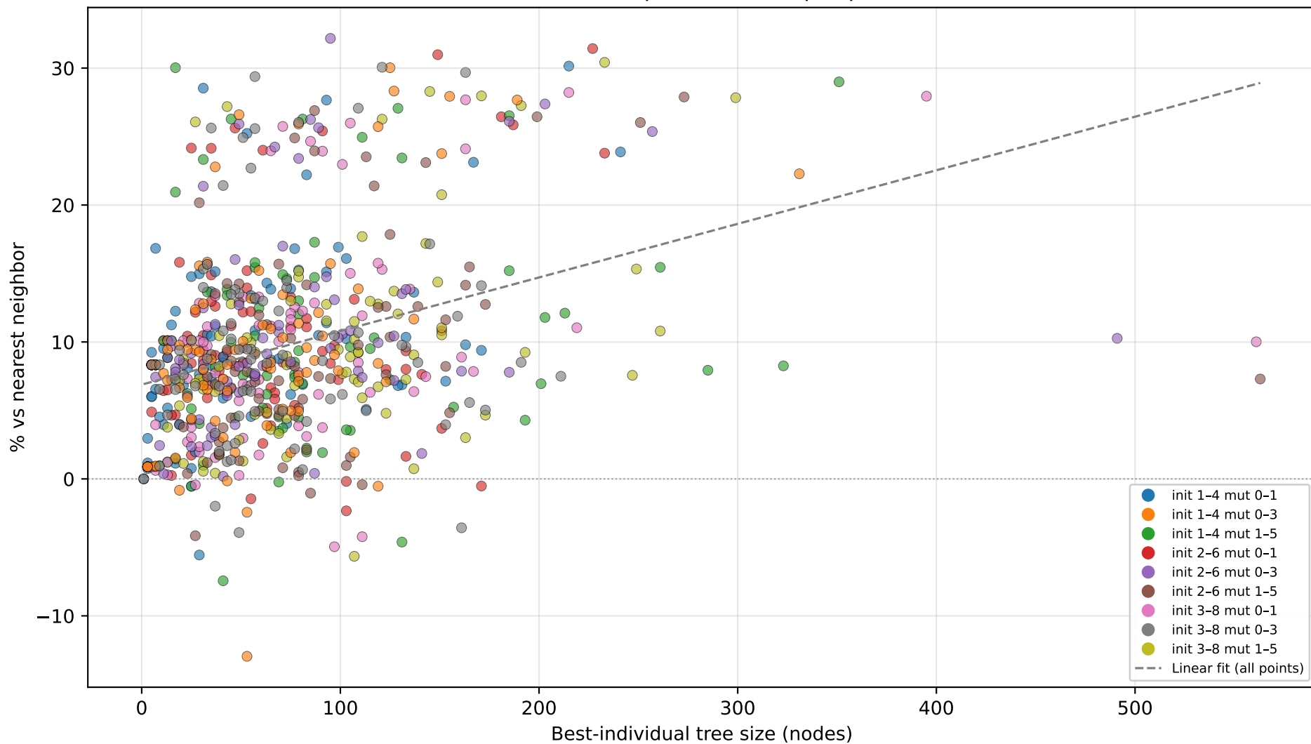
Best-individual tree size vs GP performance (per problem variant x run)
