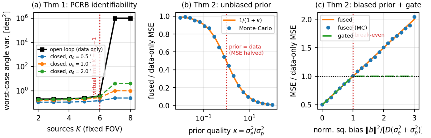
Fig. 5: Validation of the two central theorems. (a) Theorem 1: the open-loop bound diverges at the virtual-array limit K=M_v-1 while the closed-loop PCRB stays finite, bounded by the prior information (near-parity when well-determined). (b) Theorem 2, unbiased prior: the fused subspace MSE follows 1/(1+\kappa) . (c) Theorem 2, biased prior: the break-even is exactly \|b\|^2 = D(\sigma_e^2 + \sigma_p^2) , where the gated estimator clamps to and never exceeds the data-only MSE.
