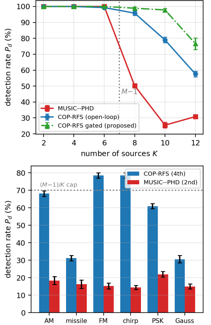
Fig. 3: Robustness sweeps (20 trials, 95% CIs). Top : end-to-end detection P_d vs. source count K ( M = 8 , near-stationary)—MUSIC collapses past M-1=7 while COP and the proposed gated loop degrade gracefully. Bottom : P_d vs. source signal type at K = 10 > M-1 —the higher-order front-end holds for structured non-Gaussian radar/comm waveforms and degrades, as predicted, for purely Gaussian sources (vanishing 4th cumulant) and severely fluctuating Swerling returns.
