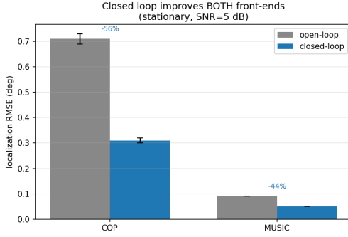
Fig. 4: Closed-loop refinement improves both the cumulant (COP) and covariance (MUSIC) front-ends (stationary, SNR= 5 dB, K = 6 ). Bars: matched-pair localization RMSE; error bars are 95% CIs.
