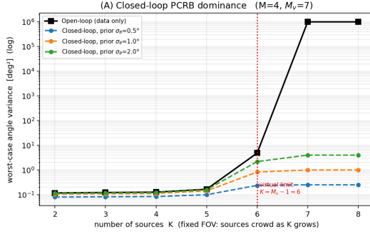
Fig. 6: Validation of Theorem 1: open-loop bound diverges at the virtual-array limit while the closed-loop PCRB stays finite; near-parity in the well-determined regime.
