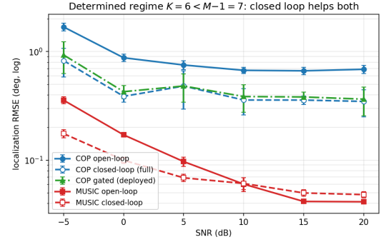
Fig. 5: Determined regime ( K = 6 < M-1 ): localization RMSE vs. SNR for COP and MUSIC (open- and closed-loop) plus the deployed gated COP (GCL), which overlaps the full closed loop (30 trials, 95% CIs). The closed loop helps both front-ends—most at low SNR—and helps COP at every SNR because its higher-order variance keeps the prior informative.
