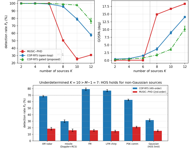
Fig. 3: Robustness sweeps (20 trials, 95% CIs). Top : end-to-end detection P_d and GOSPA vs. source count K ( M = 8 , near-stationary)—MUSIC collapses past M - 1 = 7 while COP and the proposed gated loop degrade gracefully. Bottom : P_d vs. source signal type at K = 10 > M - 1 —the higher-order front-end holds for structured non-Gaussian radar/comm waveforms and degrades, as predicted, for purely Gaussian sources (vanishing 4th cumulant) and severely fluctuating Swerling returns.
