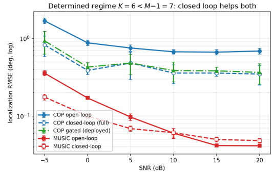
Fig. 6: Determined regime ( K = 6 < M-1 ): localization RMSE vs. SNR for COP and MUSIC (open- and closed-loop) plus the deployed gated COP (GCL), which overlaps the full closed loop (30 trials, 95% CIs). The closed loop helps both front-ends—most at low SNR—and helps COP at every SNR because its higher-order variance keeps the prior informative.
