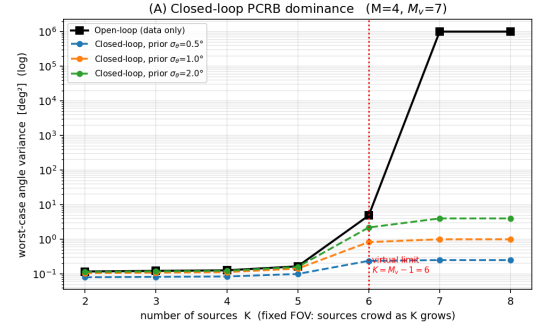
Fig. 7: Validation of Theorem 1: open-loop bound diverges at the virtual-array limit while the closed-loop PCRB stays finite; near-parity in the well-determined regime.
