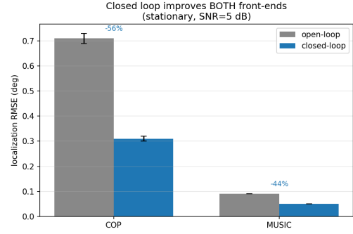
Fig. 5: Closed-loop refinement improves both the cumulant (COP) and covariance (MUSIC) front-ends (stationary, SNR= 5 dB, K = 6 ). Bars: matched-pair localization RMSE; error bars are 95% CIs.
