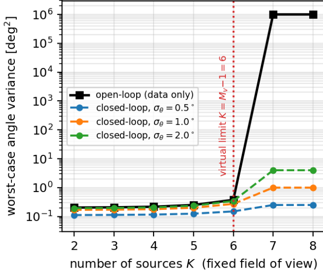
Fig. 5: Validation of Theorem 1: the open-loop bound diverges at the virtual-array limit K=M_v-1 while the closed-loop PCRb stays finite, bounded by the prior information; near-parity in the well-determined regime.
