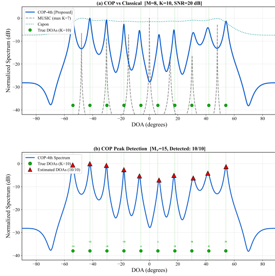
Fig. 2: Spatial spectrum for K = 10 sources, M = 8 ( K > M-1 = 7 ): COP-4th resolves all sources via the virtual aperture, while MUSIC and Capon fail. (Top) pseudo-spectra; (bottom) COP peak detection.
