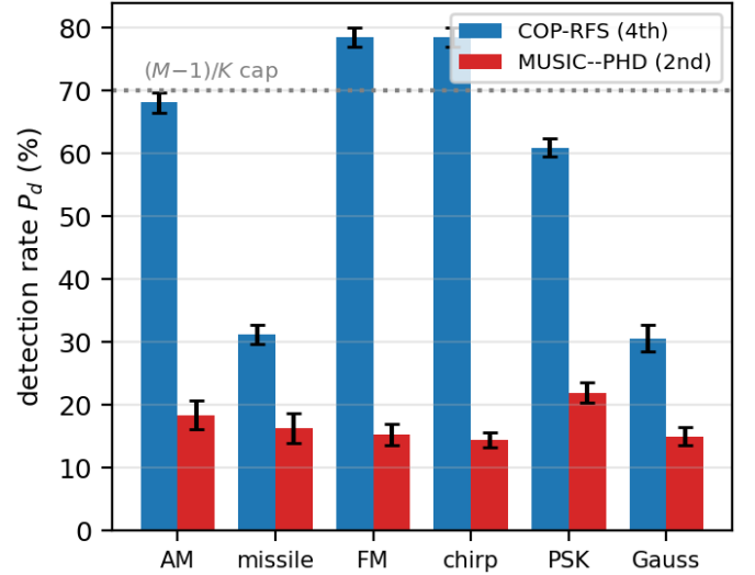
Fig. 3: Robustness sweeps (20 trials, 95% CIs). Top : end-to-end detection P_d vs. source count K ( M = 8 , near-stationary)—MUSIC collapses past M-1=7 while COP and the proposed gated loop degrade gracefully. Bottom : P_d vs. source signal type at K = 10 > M-1 —the higher-order front-end holds for structured non-Gaussian radar/comm waveforms and degrades, as predicted, for purely Gaussian sources (vanishing 4th cumulant) and severely fluctuating Swerling returns.
