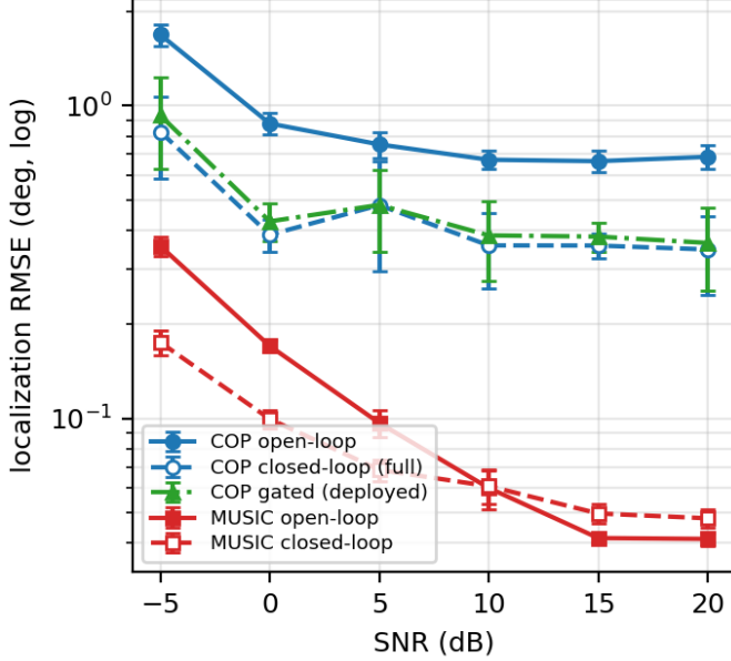
Fig. 4: Determined regime ( K = 6 < M-1 ): localization RMSE vs. SNR for COP and MUSIC (open- and closed-loop) plus the deployed gated closed loop (GCL), which overlaps the full closed loop (30 trials, 95% CIs). The closed loop helps both front-ends—most at low SNR—and helps COP at every SNR because its higher-order variance keeps the prior informative.
