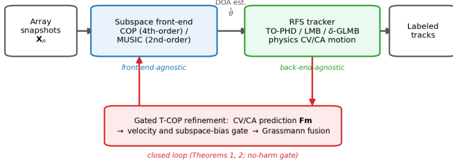
Fig. 1: The proposed gated closed-loop subspace-RFS framework. A front-end-agnostic subspace estimator (COP or MUSIC) feeds a back-end-agnostic RFS tracker (TO-PHD, LMB, or \delta -GLMB with physics-based CV/CA motion); the tracker’s prediction is fed back through a validation gate and a minimum-variance T-COP refinement (Theorems 1–2) that guarantees the loop never degrades the open-loop estimate. The recommended deployed configuration is a gated COP front-end driving a physics-based \delta -GLMB back-end.
