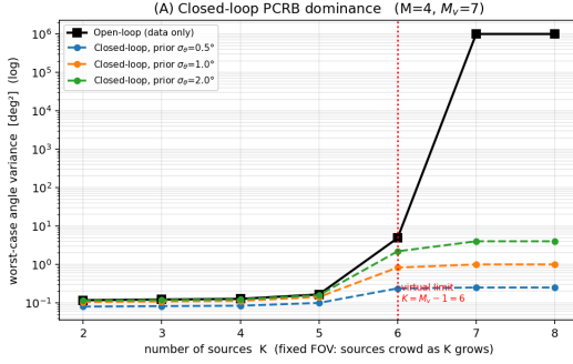
Fig. 7: Validation of Theorem 1: open-loop bound diverges at the virtual-array limit while the closed-loop PCRB stays finite; near-parity in the well-determined regime.
