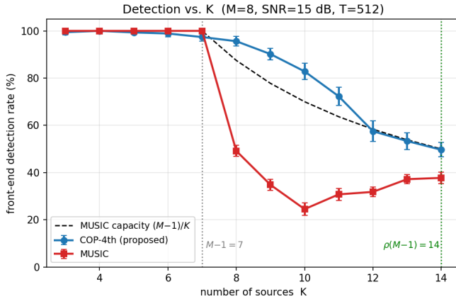
Fig. 2: Front-end detection rate vs. source count K ( M = 8 , \text{SNR} = 15 dB, T = 512 , 60 trials, 95% CIs). MUSIC collapses for K > M - 1 = 7 toward its (M - 1)/K capacity, while COP-4th sustains detection up to the virtual-array limit \rho(M - 1) = 14 .
