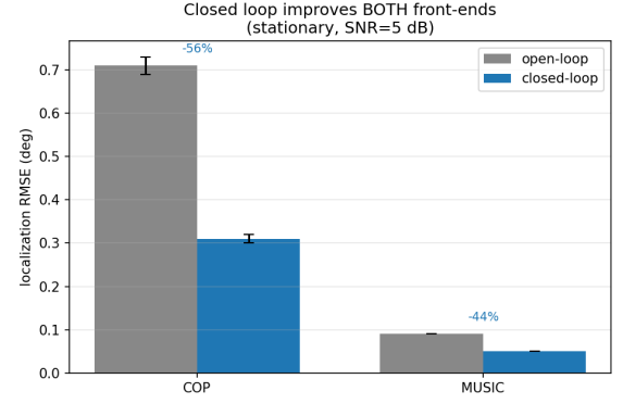
Fig. 3: Closed-loop refinement improves both the cumulant (COP) and covariance (MUSIC) front-ends (stationary, \text{SNR} = 5 dB, K = 6 ). Bars: matched-pair localization RMSE; error bars are 95% CIs.
