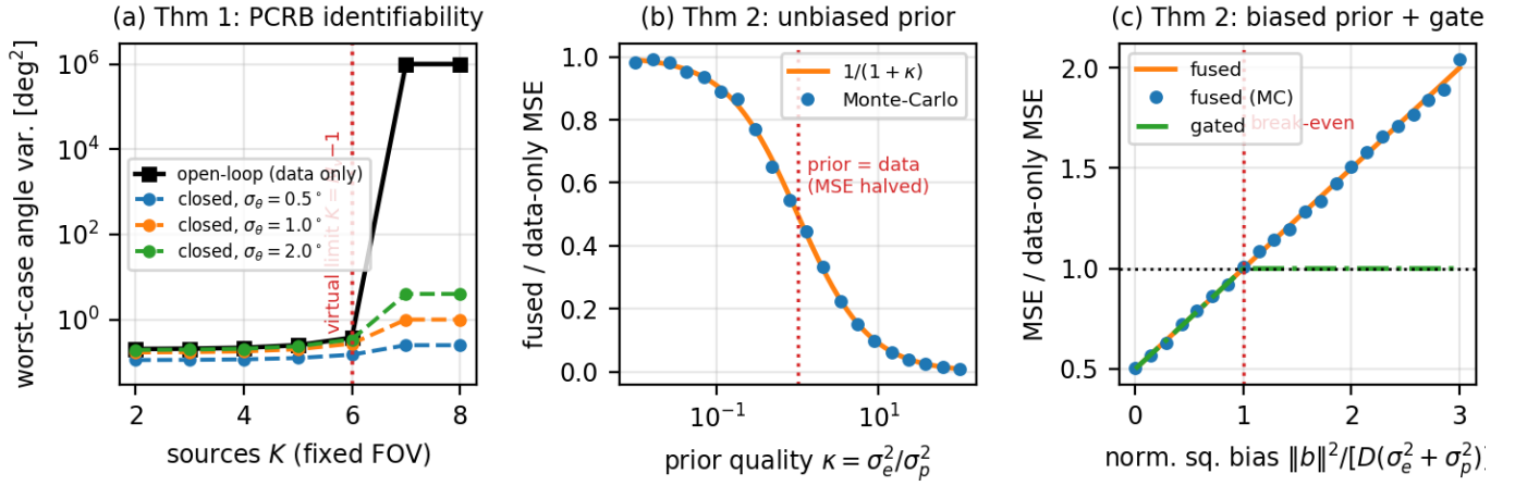
Fig. 5: Validation of the two central theorems. (a) Theorem 1: the open-loop bound diverges at the virtual-array limit K = M_v - 1 while the closed-loop PCRB stays finite, bounded by the prior information (near-parity when well-determined). (b) Theorem 2, unbiased prior: the fused subspace MSE follows 1/(1 + \kappa) . (c) Theorem 2, biased prior: the break-even is exactly \|b\|^2 = D(\sigma_e^2 + \sigma_p^2) , where the gated estimator clamps to and never exceeds the data-only MSE.
