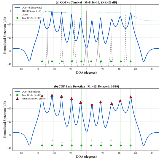
Fig. 2: Spatial spectrum for K = 10 sources, M = 8 ( K > M - 1 = 7 ): COP-4th resolves all sources via the virtual aperture, while MUSIC and Capon fail. (Top) pseudo-spectra; (bottom) COP peak detection.
