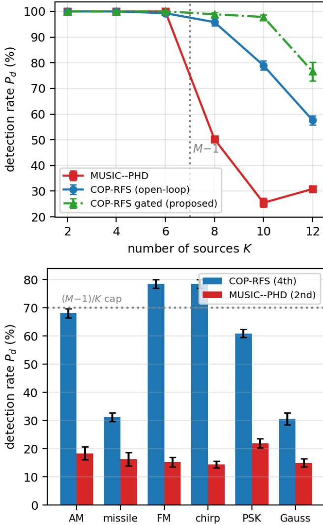
Fig. 3: Robustness sweeps (20 trials, 95% CIs). Top : end-to-end detection P_d vs. source count K ( M = 8 , near-stationary)—MUSIC collapses past M-1=7 while COP and the proposed gated loop degrade gracefully. Bottom : P_d vs. source signal type at K = 10 > M-1 —the higher-order front-end holds for structured non-Gaussian radar/comm waveforms and degrades, as predicted, for purely Gaussian sources (vanishing 4th cumulant) and severely fluctuating Swerling returns.
