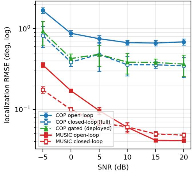
Fig. 4: Determined regime ( K = 6 < M-1 ): localization RMSE vs. SNR for COP and MUSIC (open- and closed-loop) plus the deployed gated closed loop (GCL), which overlaps the full closed loop (30 trials, 95% CIs). The closed loop helps both front-ends—most at low SNR—and helps COP at every SNR because its higher-order variance keeps the prior informative.
