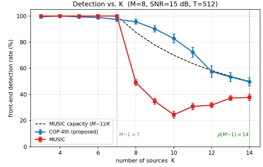
Fig. 3: Front-end detection rate vs. source count K ( M = 8 , SNR=15 dB, T = 512 , 60 trials, 95% CIs). MUSIC collapses for K > M-1 = 7 toward its (M-1)/K capacity, while COP-4th sustains detection up to the virtual-array limit \rho(M-1) = 14 .
