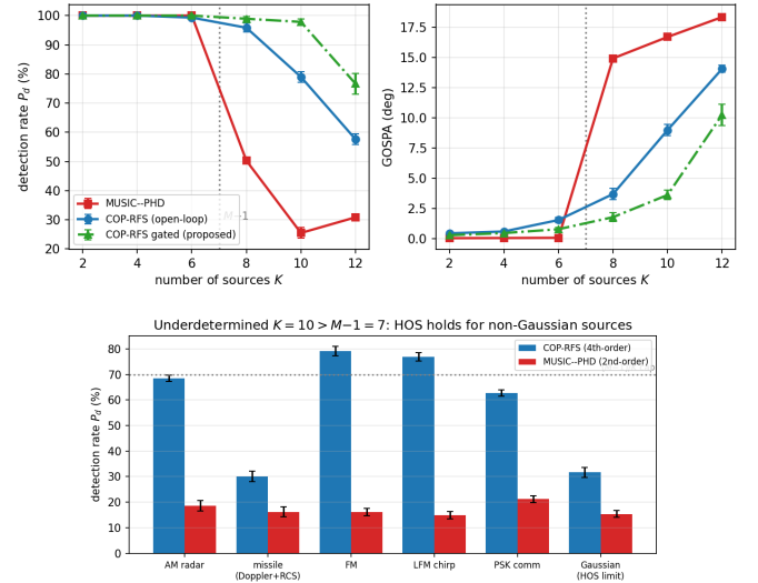
Fig. 3: Robustness sweeps (20 trials, 95% CIs). Top : end-to-end detection P_d and GOSPA vs. source count K ( M = 8 , near-stationary)—MUSIC collapses past M-1=7 while COP and the proposed gated loop degrade gracefully. Bottom : P_d vs. source signal type at K = 10 > M-1 —the higher-order front-end holds for structured non-Gaussian radar/comm waveforms and degrades, as predicted, for purely Gaussian sources (vanishing 4th cumulant) and severely fluctuating Swerling returns.
