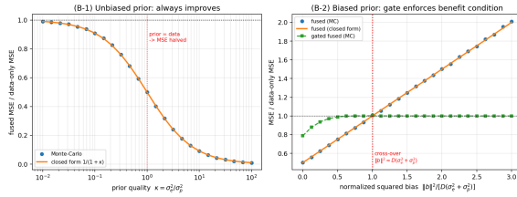
Fig. 6: Validation of Theorem 2: (left) unbiased-prior MSE follows 1/(1 + \kappa) ; (right) biased-prior break-even at \|\mathbf{b}\|^2 = D(\sigma_e^2 + \sigma_p^2) and the gated estimator never exceeds the data-only MSE.
