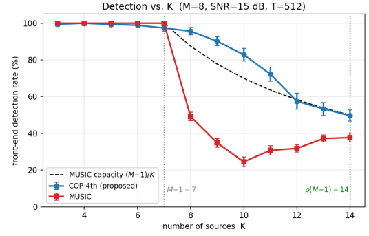
Fig. 2: Front-end detection rate vs. source count K ( M = 8 , \text{SNR} = 15 dB, T = 512 , 60 trials, 95% CIs). MUSIC collapses for K > M - 1 = 7 toward its (M - 1)/K capacity, while COP-4th sustains detection up to the virtual-array limit \rho(M - 1) = 14 .
