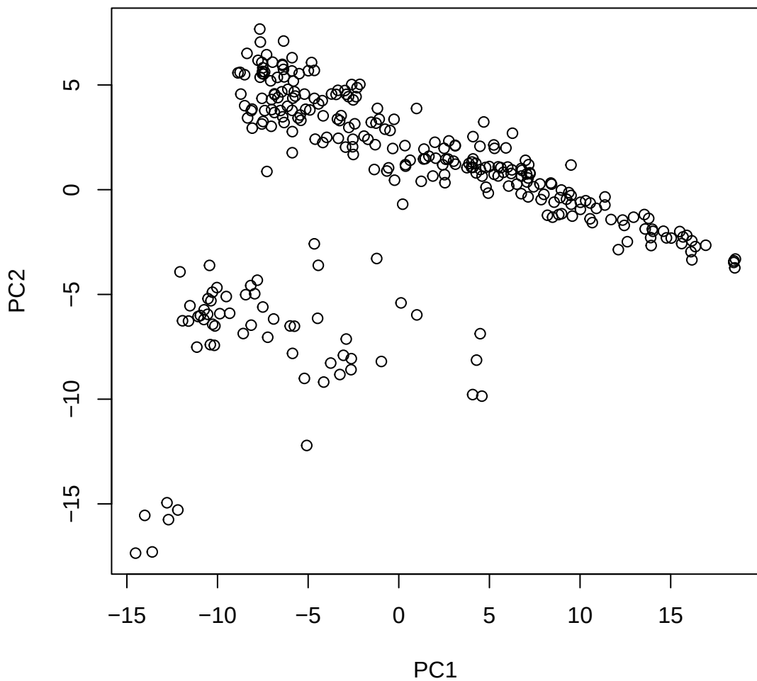
Window ID 35 NC_044051.1 (4)
