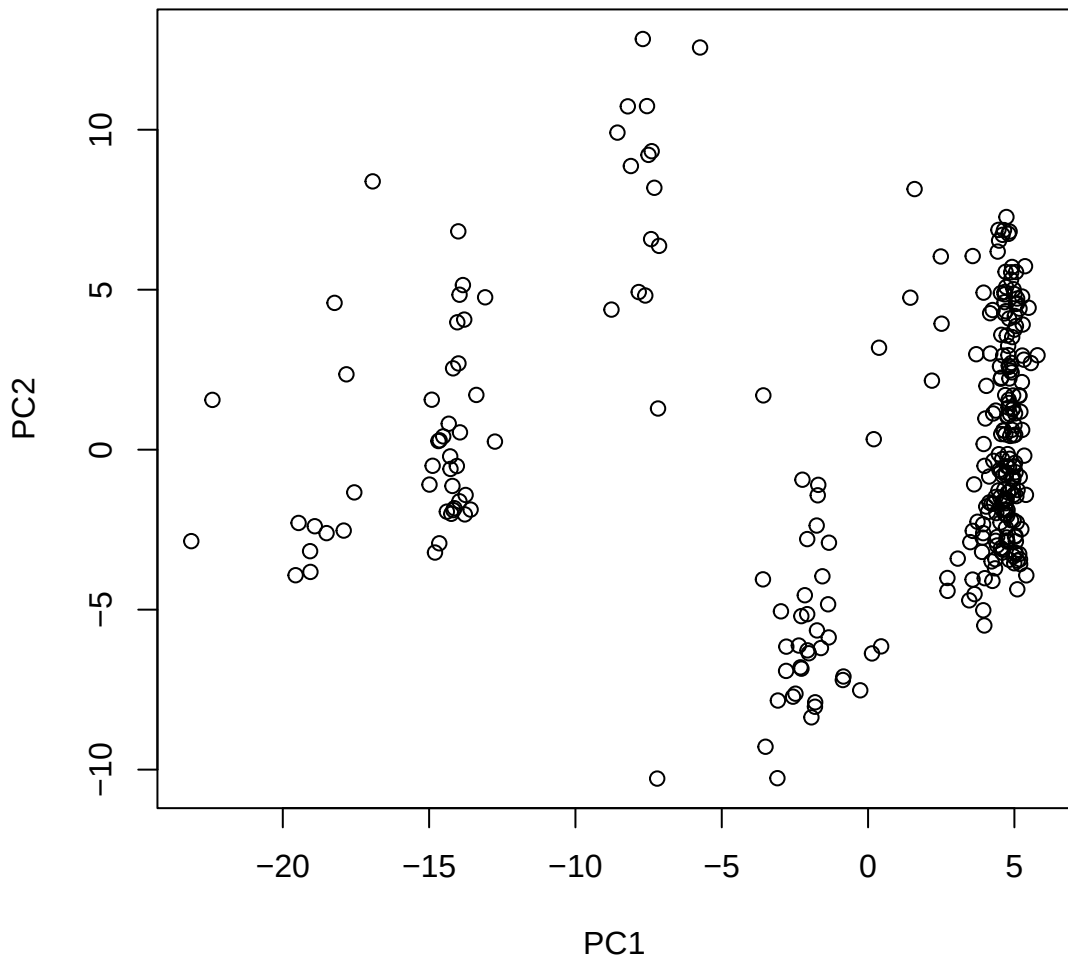
Window ID 51 NC_044053.1 (6)
