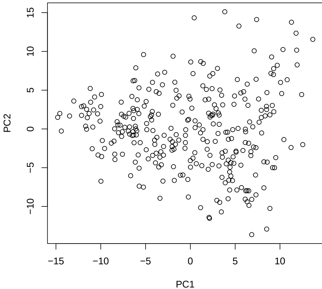
Window ID 61 NC_044054.1 (7)
