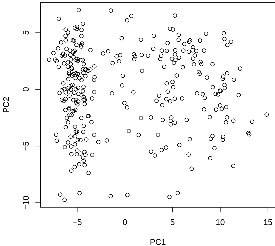
Window ID 131 NC_044061.1 (14)
