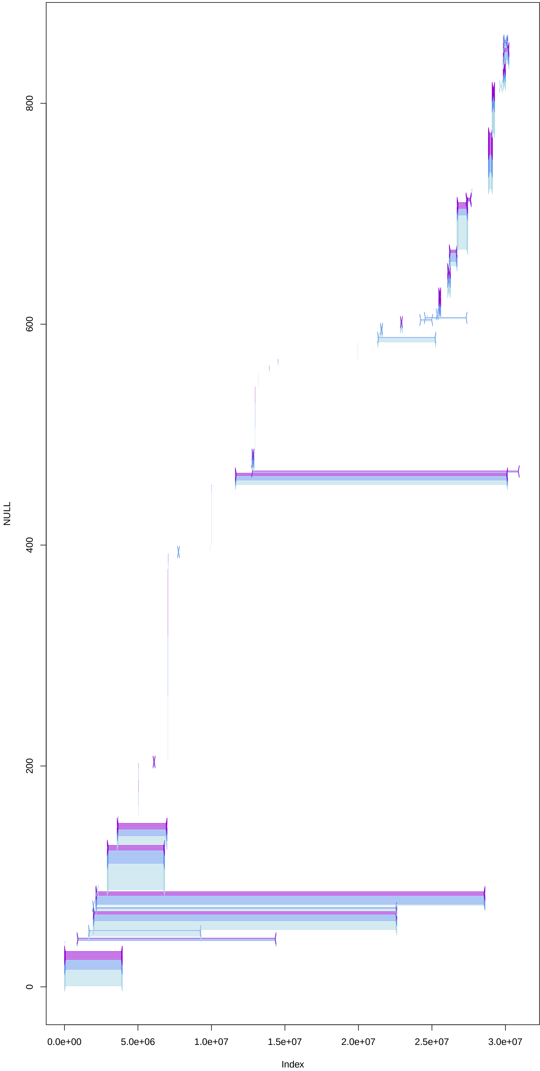
NC_044050.1 filtered 3 programs; 1 pass
