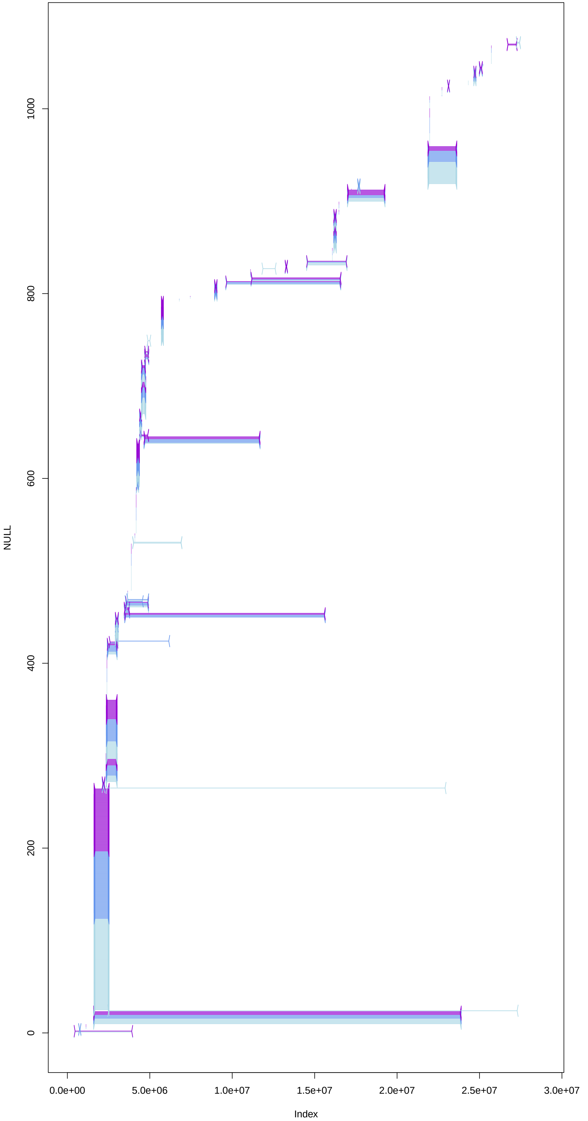
NC_044055.1 filtered 3 programs; 1 pass
