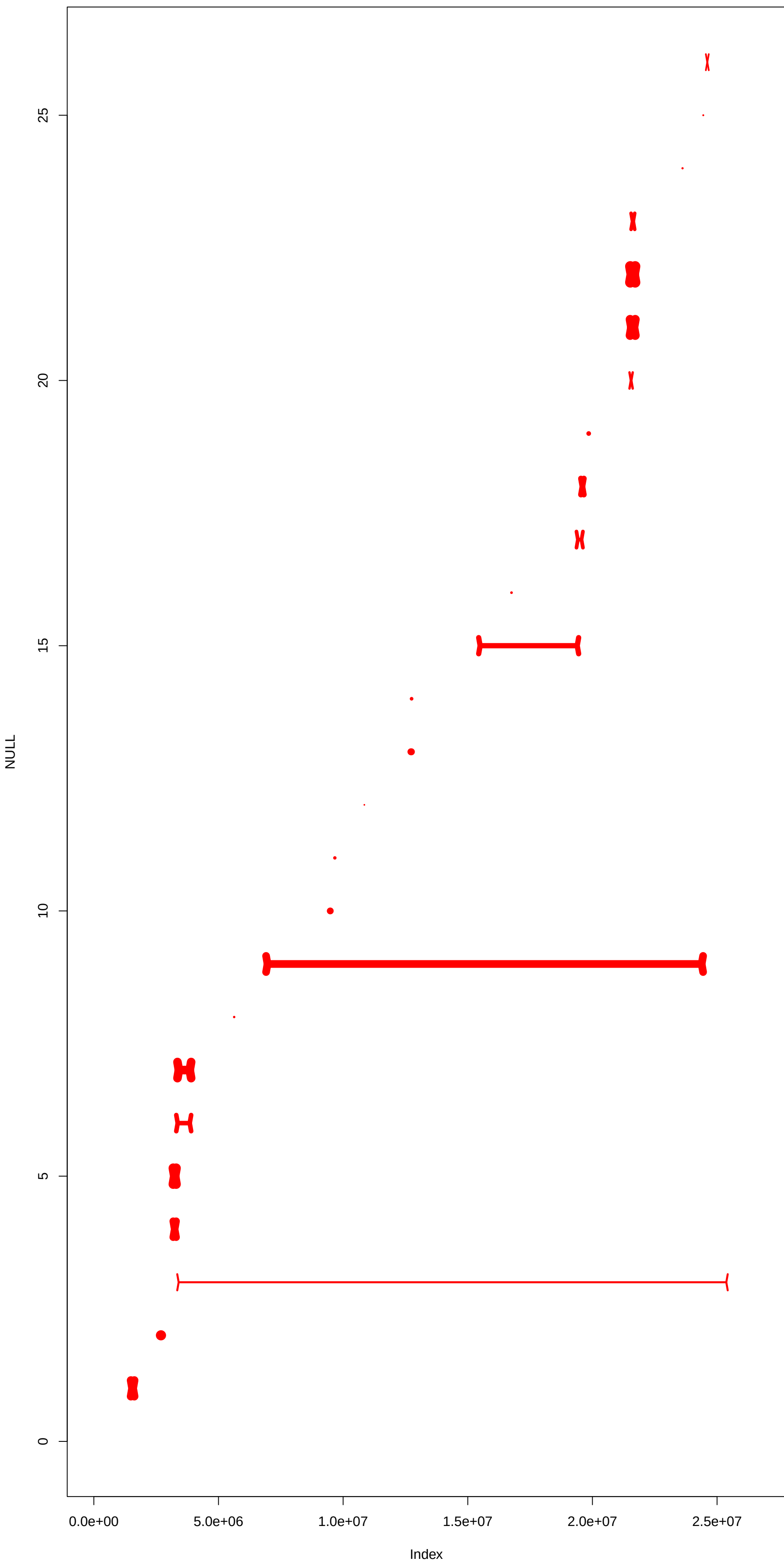
NC_044056.1 pass2
