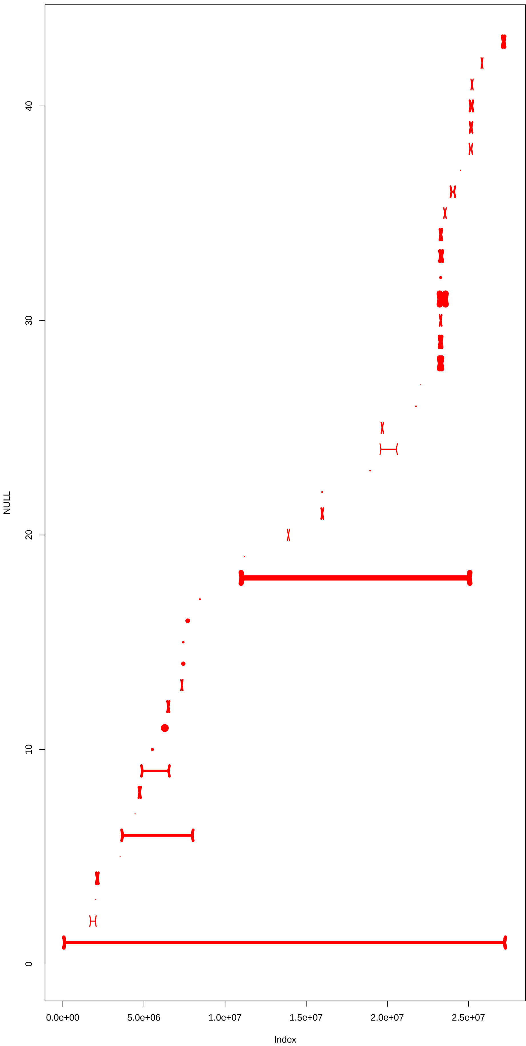
NC_044057.1 pass1
