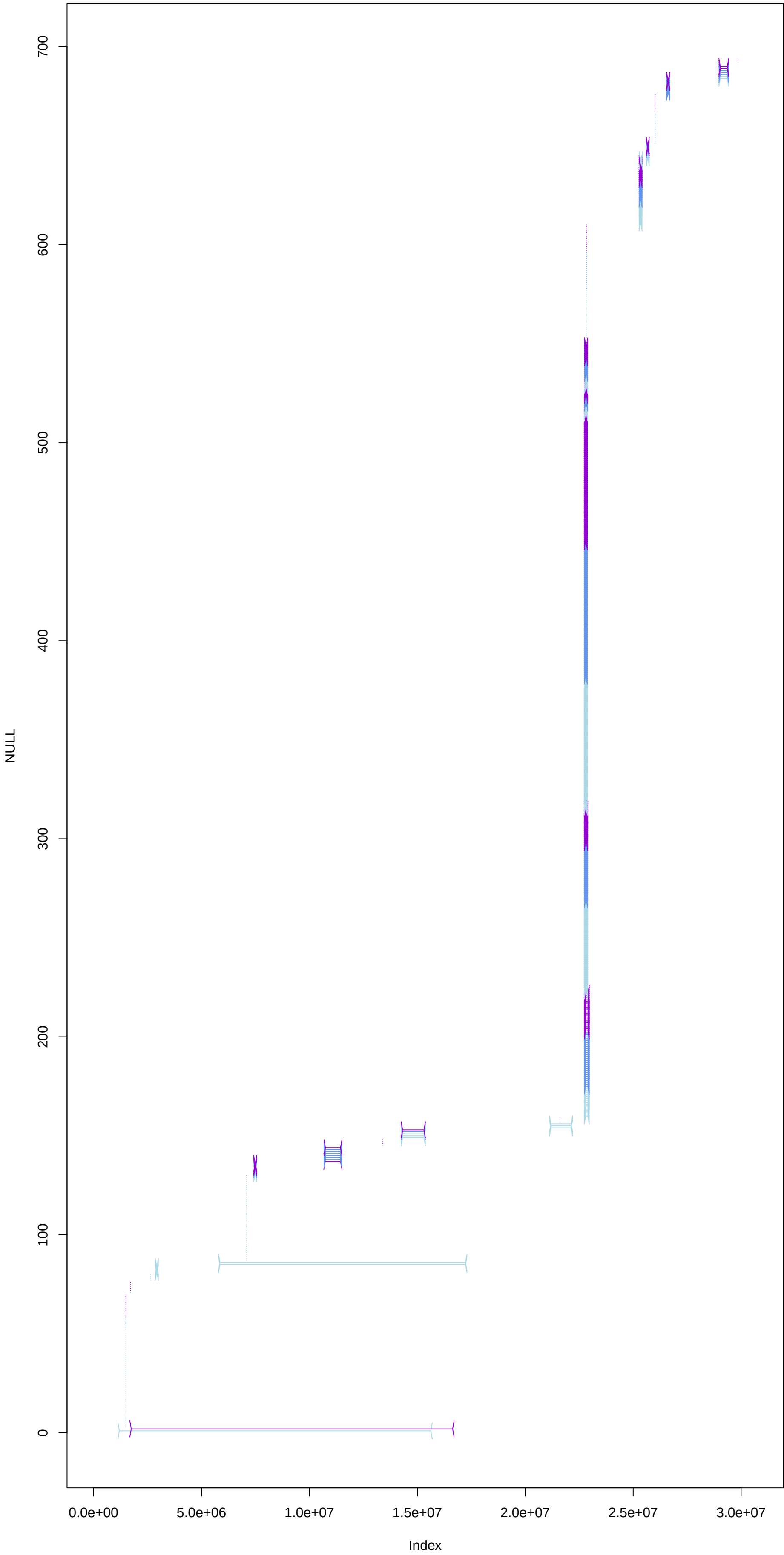
NC_044059.1 filtered 3 programs; 1 pass
