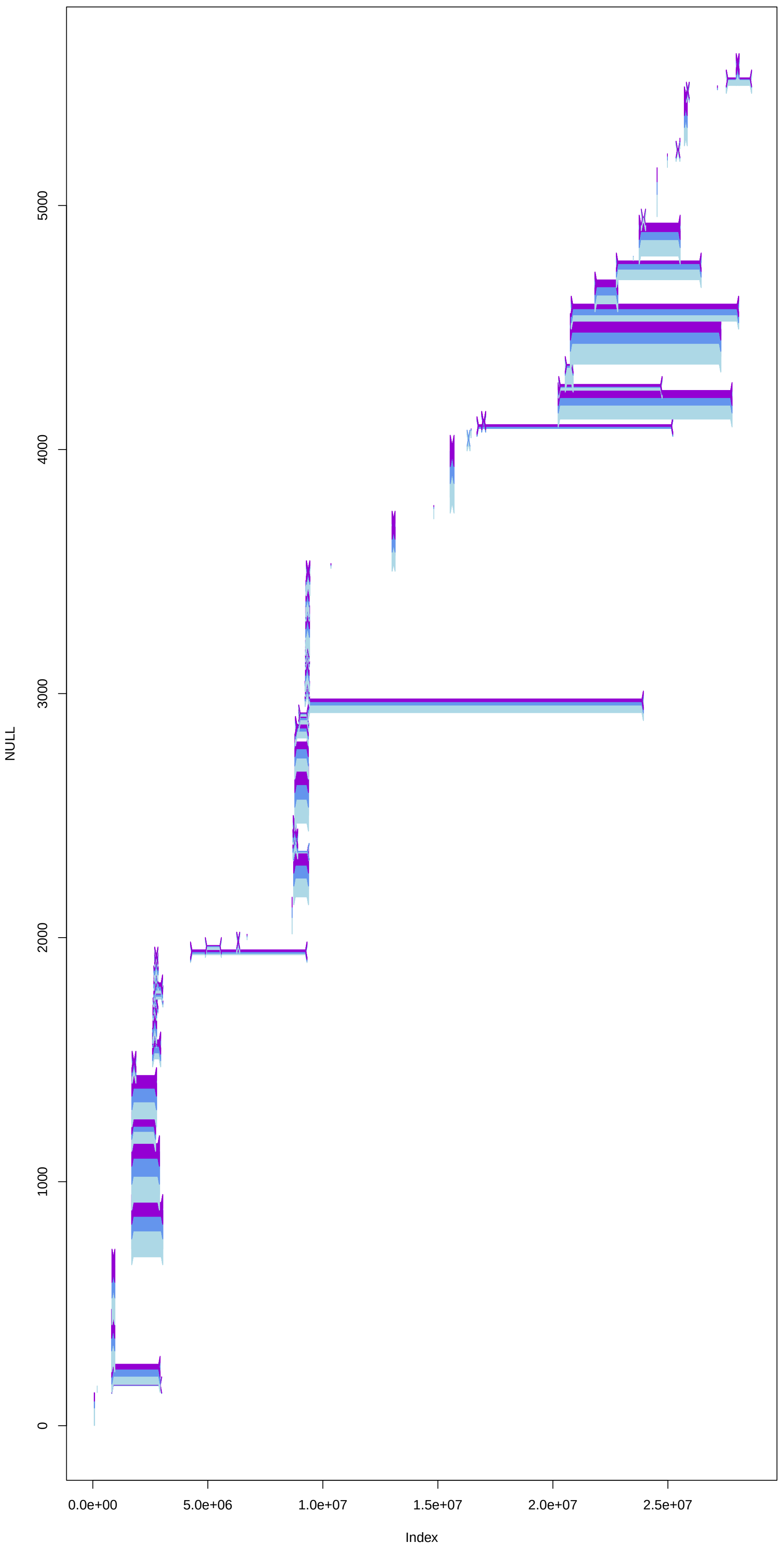
NC_044062.1
