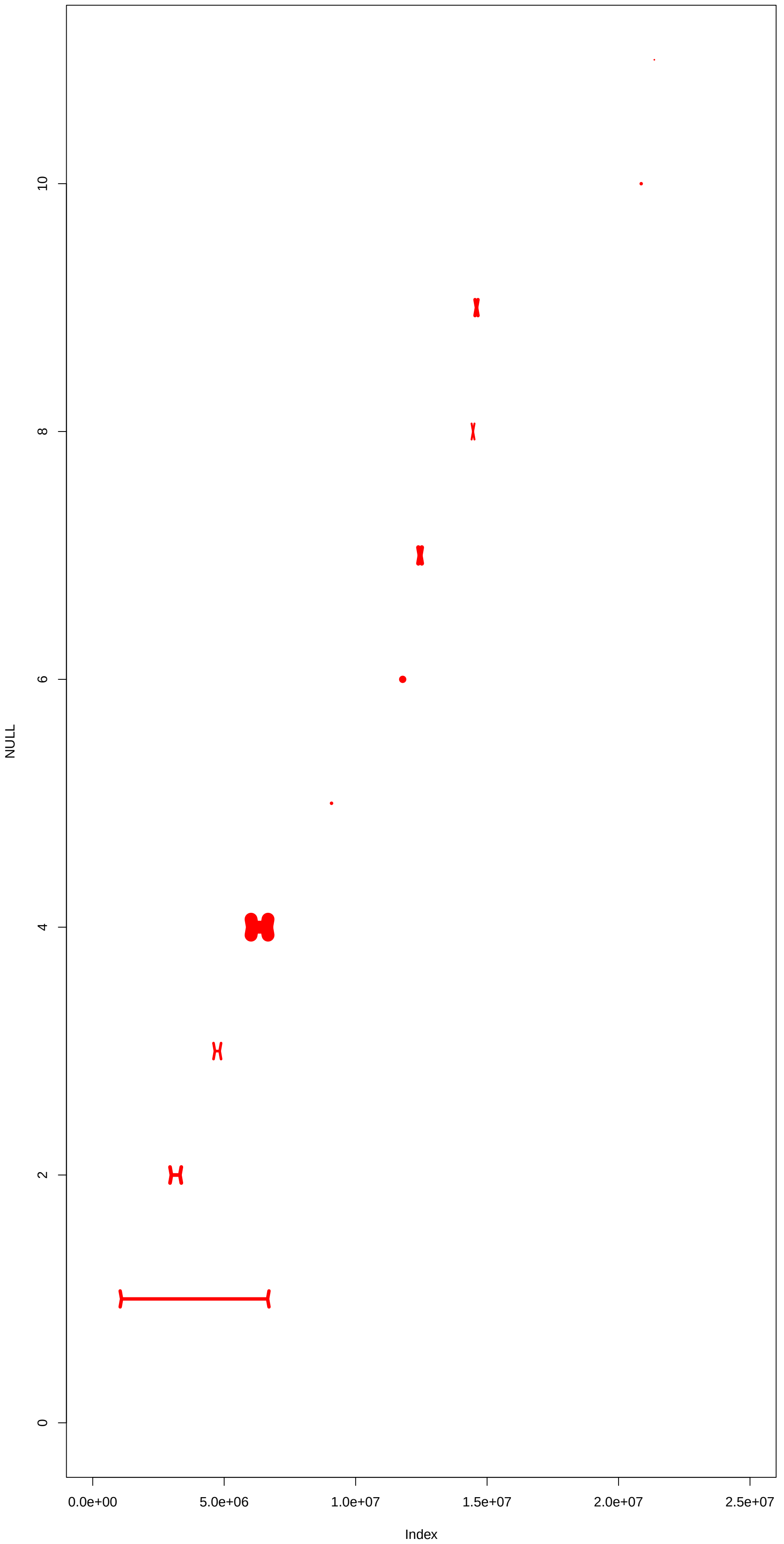
NC_044065.1 pass2
