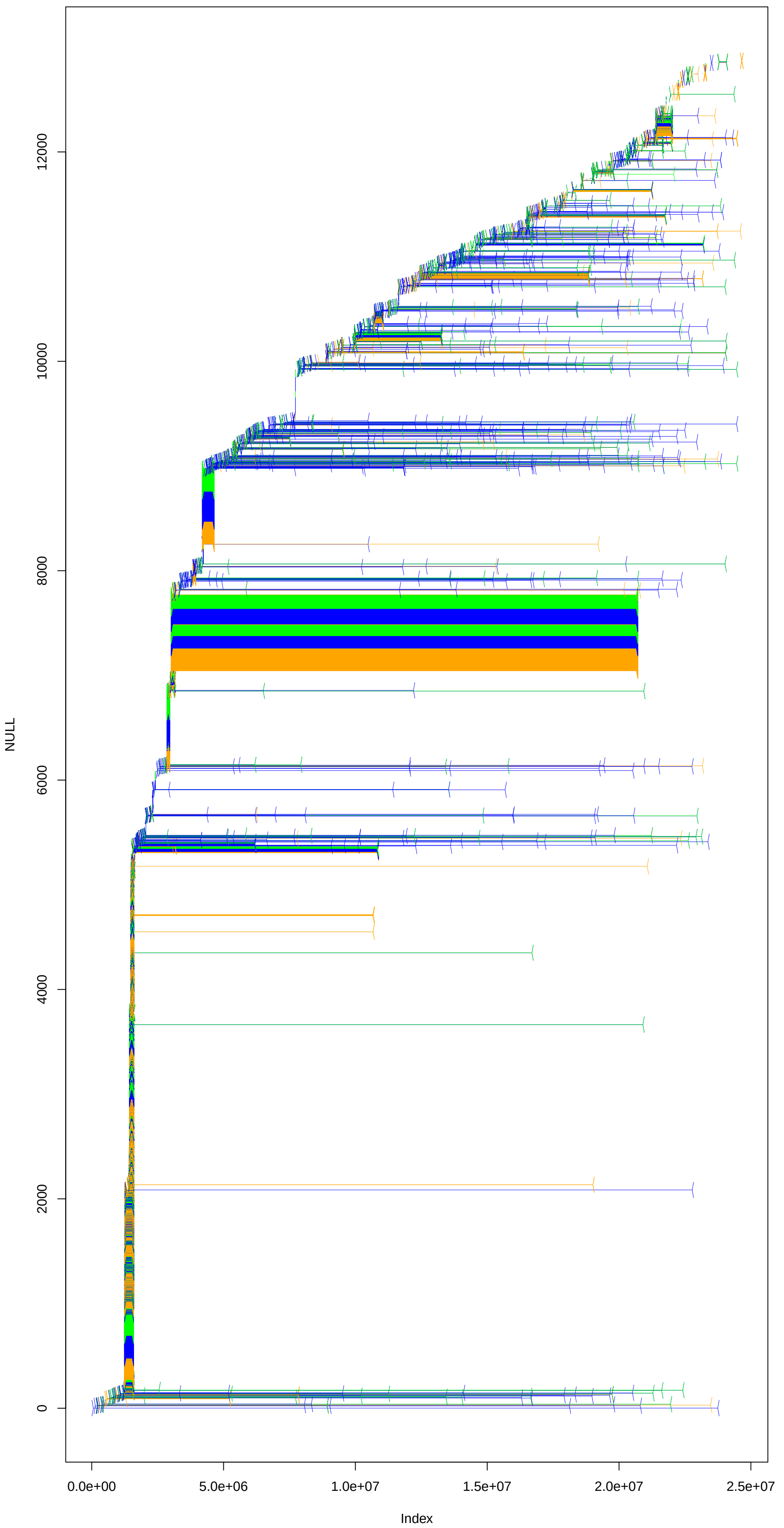
NC_044067.1
