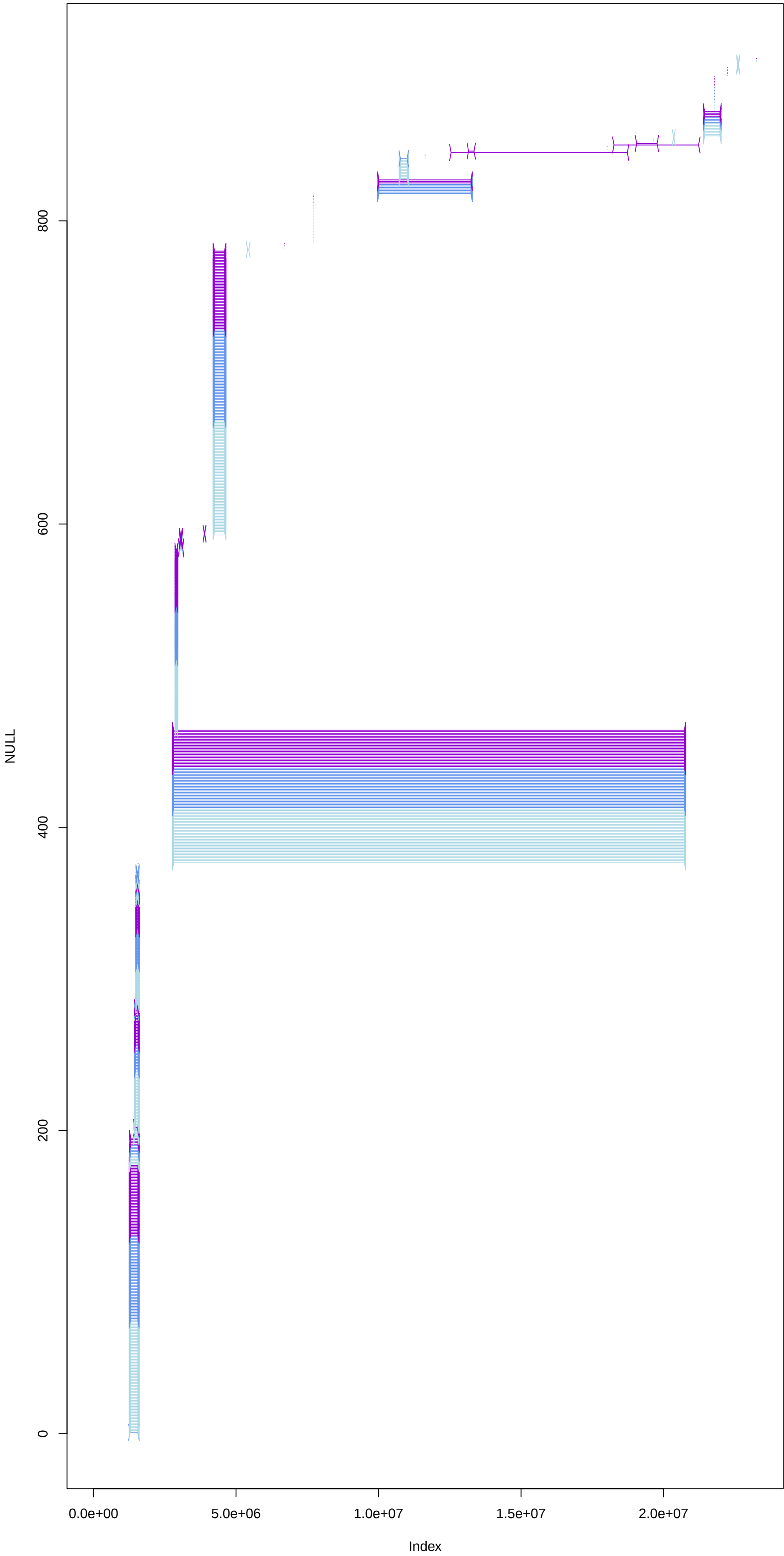
NC_044067.1 filtered 3 programs; 1 pass
