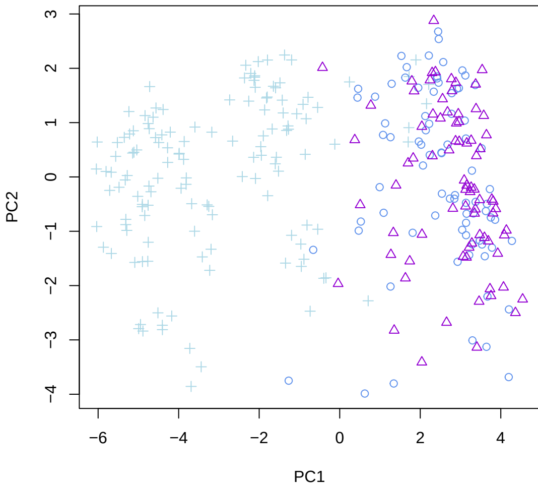
WindowID: 91; NC_044051.1 (LG 4); 99 SNPs
