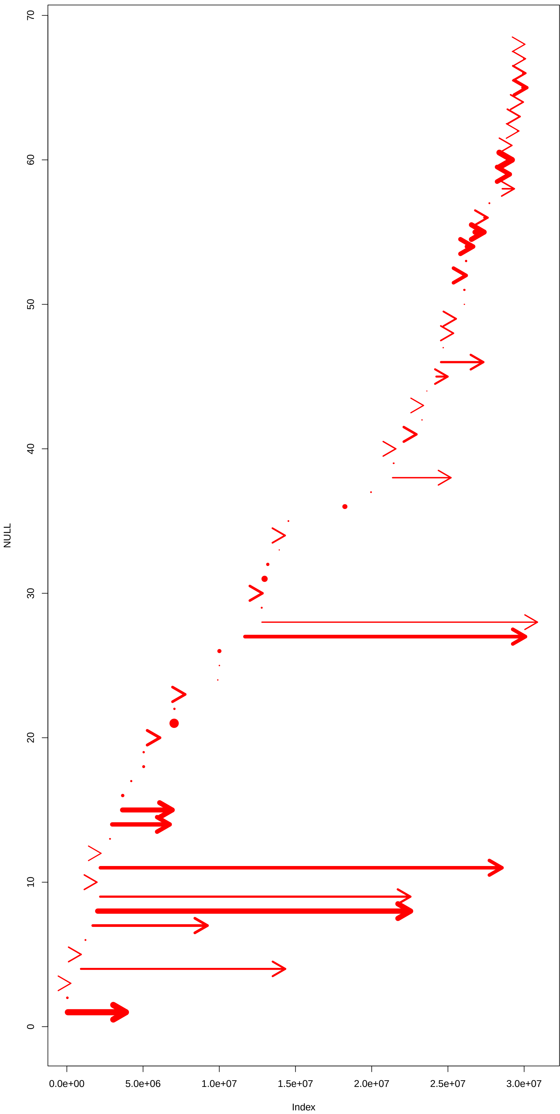
NC_044050.1
