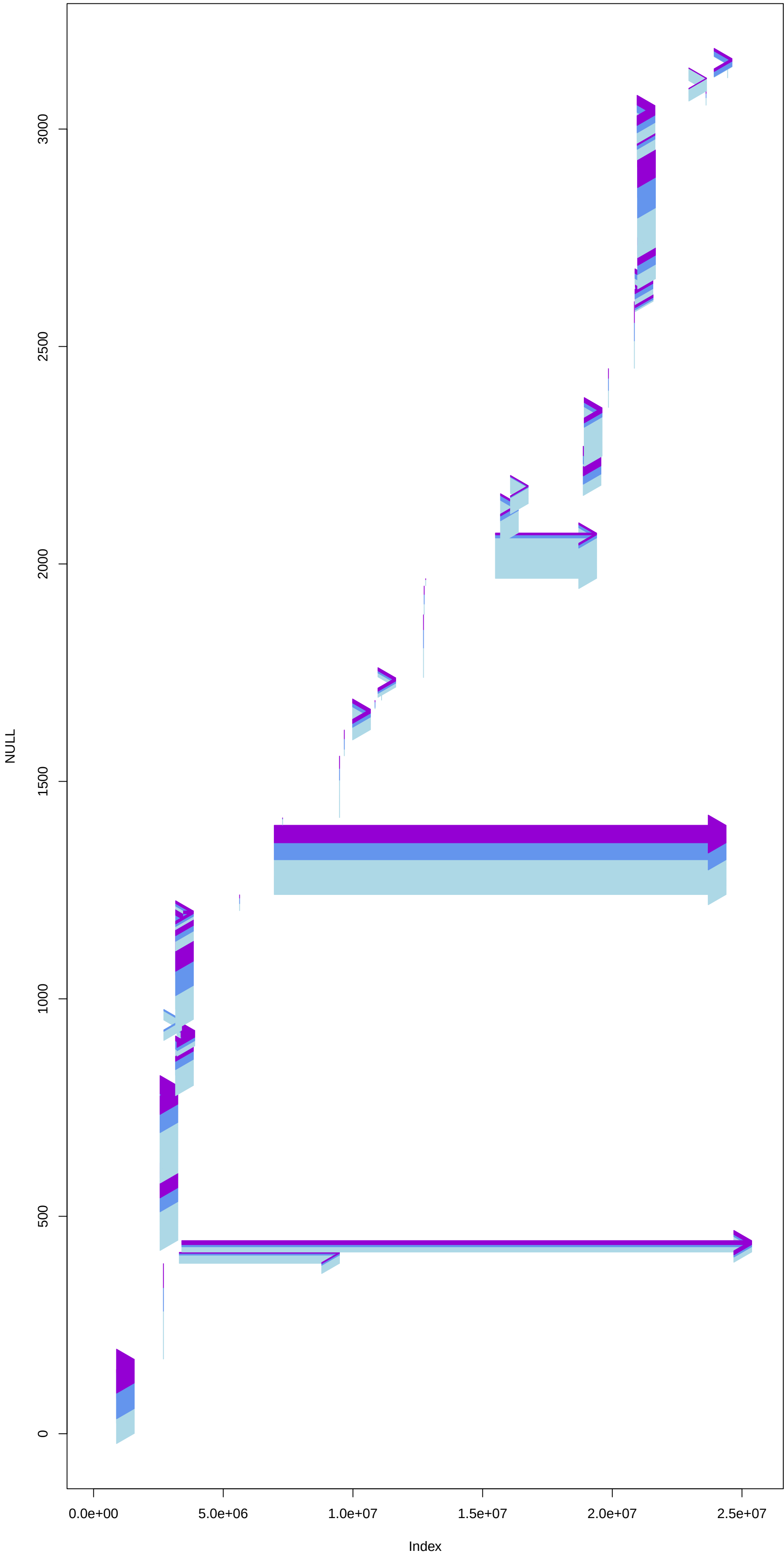
NC_044056.1
