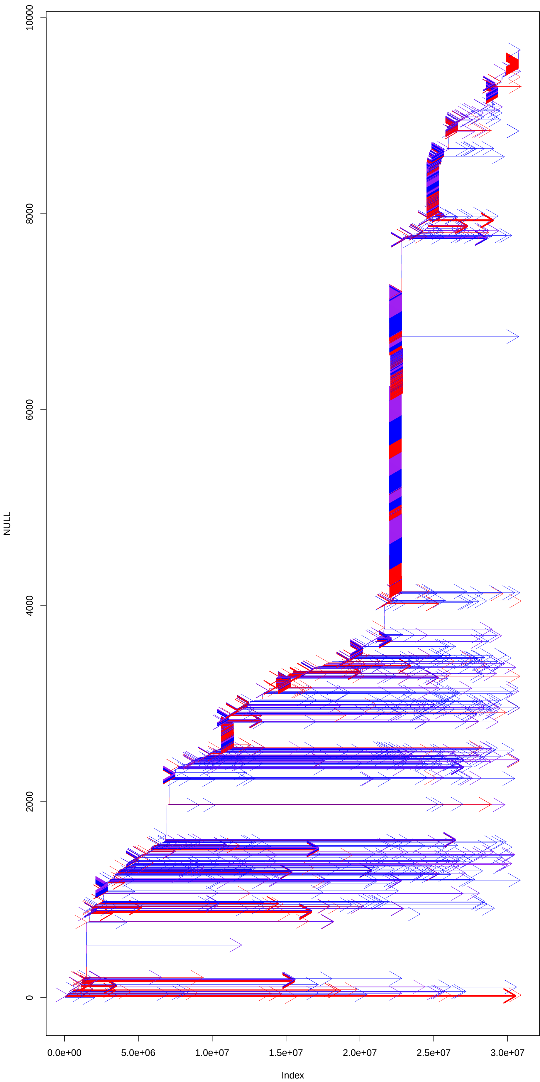
NC_044059.1
