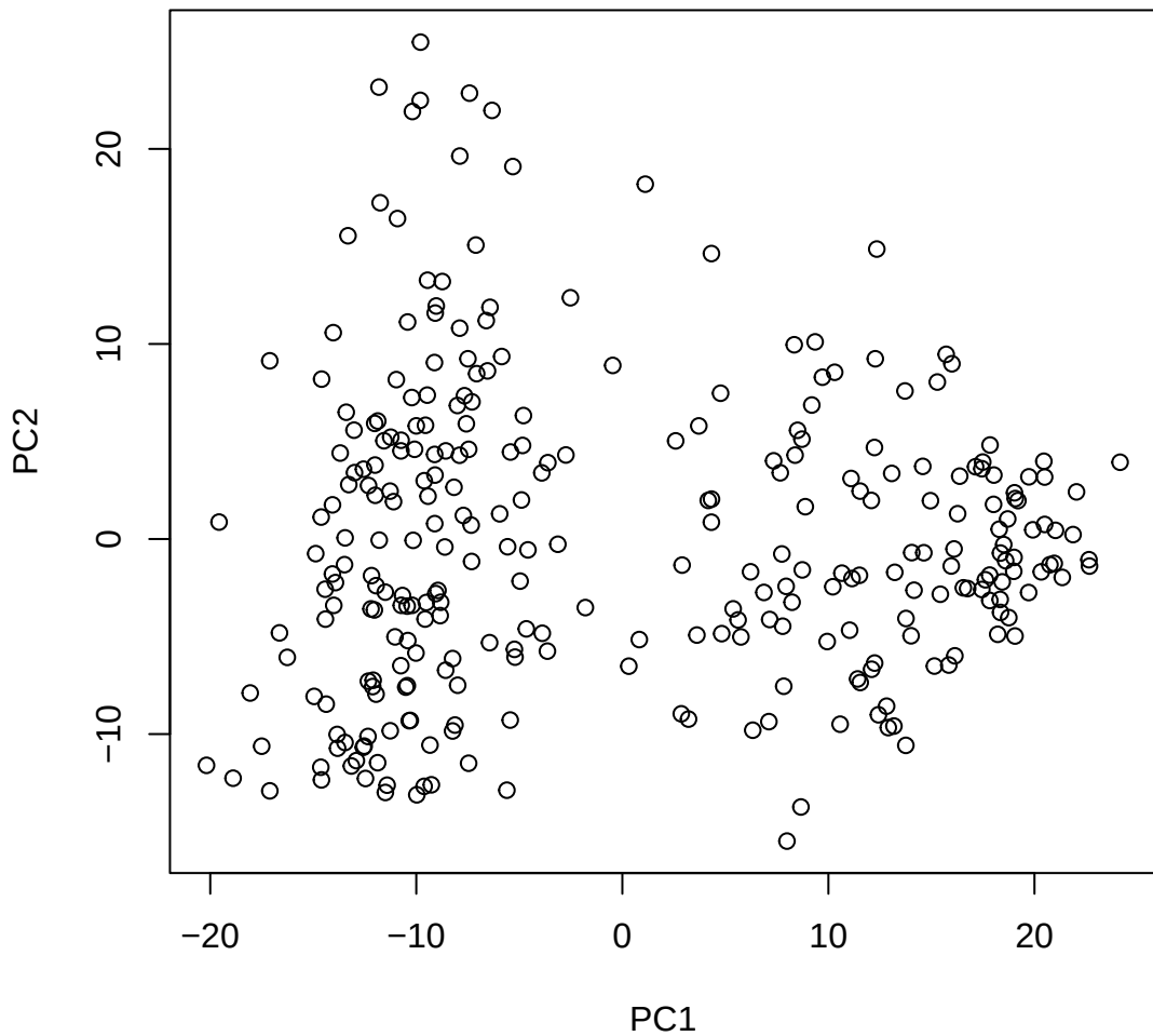
Window ID 55 NC_044053.1 (6)
