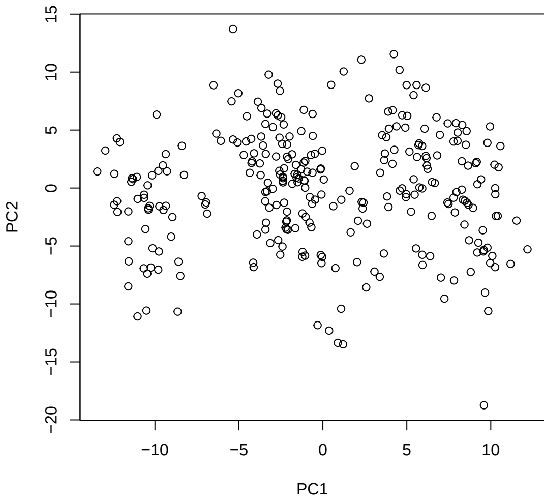
Window ID 75 NC_044055.1 (8)
