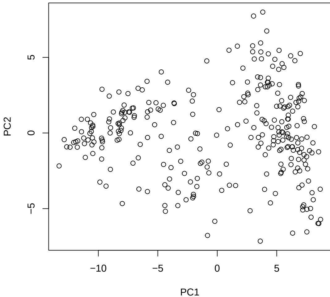
Window ID 124 NC_044061.1 (14)
