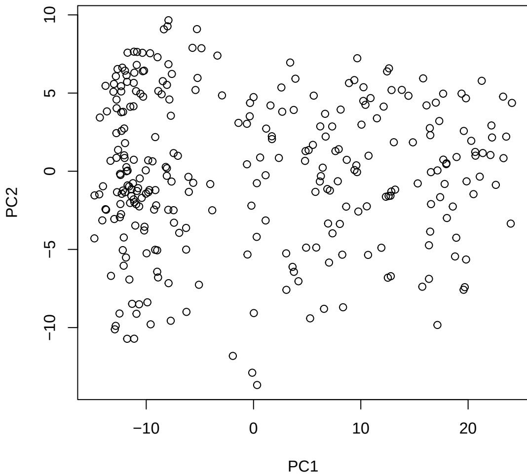
Window ID 142 NC_044063.1 (16)
