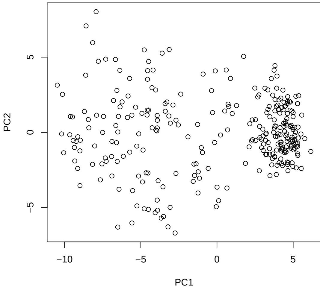
Window ID 168 NC_044066.1 (19)
