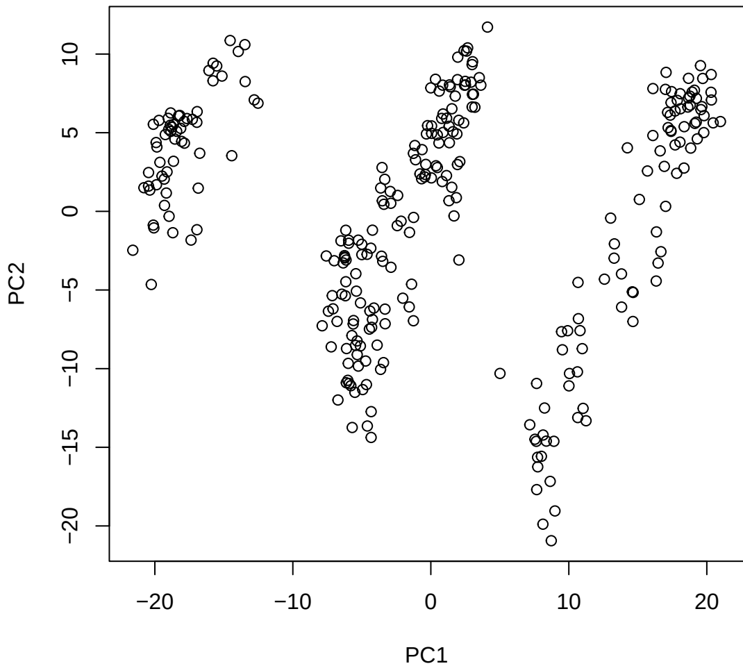
Window ID 57 NC_044054.1 (7)
