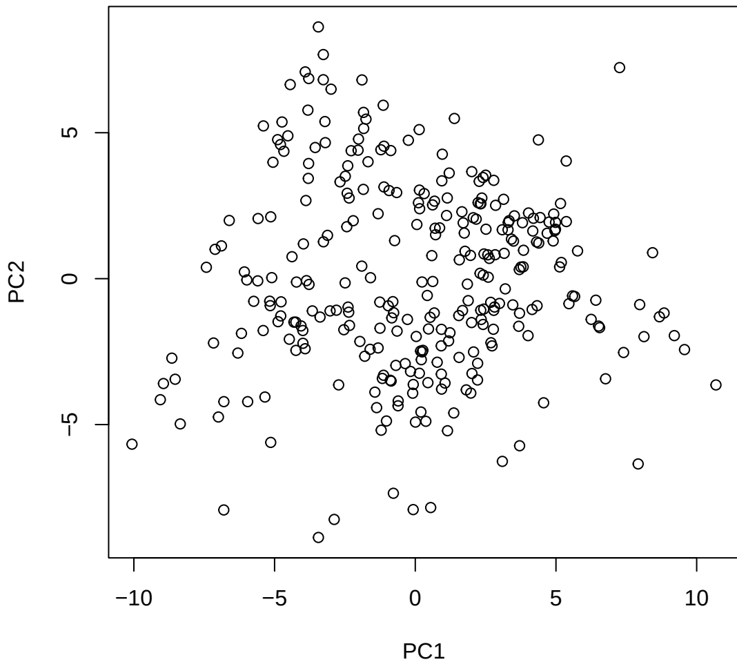
Window ID 100 NC_044057.1 (10)
