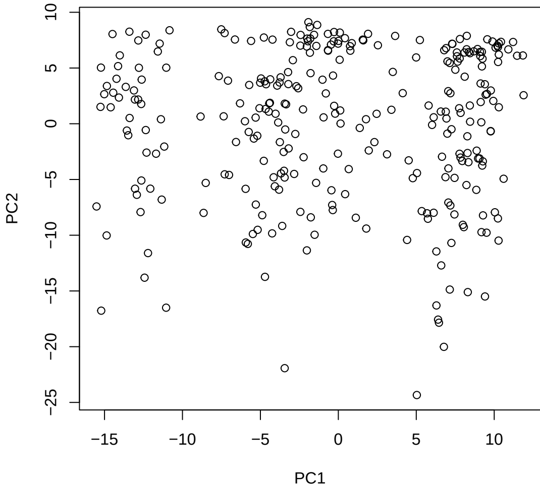
Window ID 112 NC_044059.1 (12)
