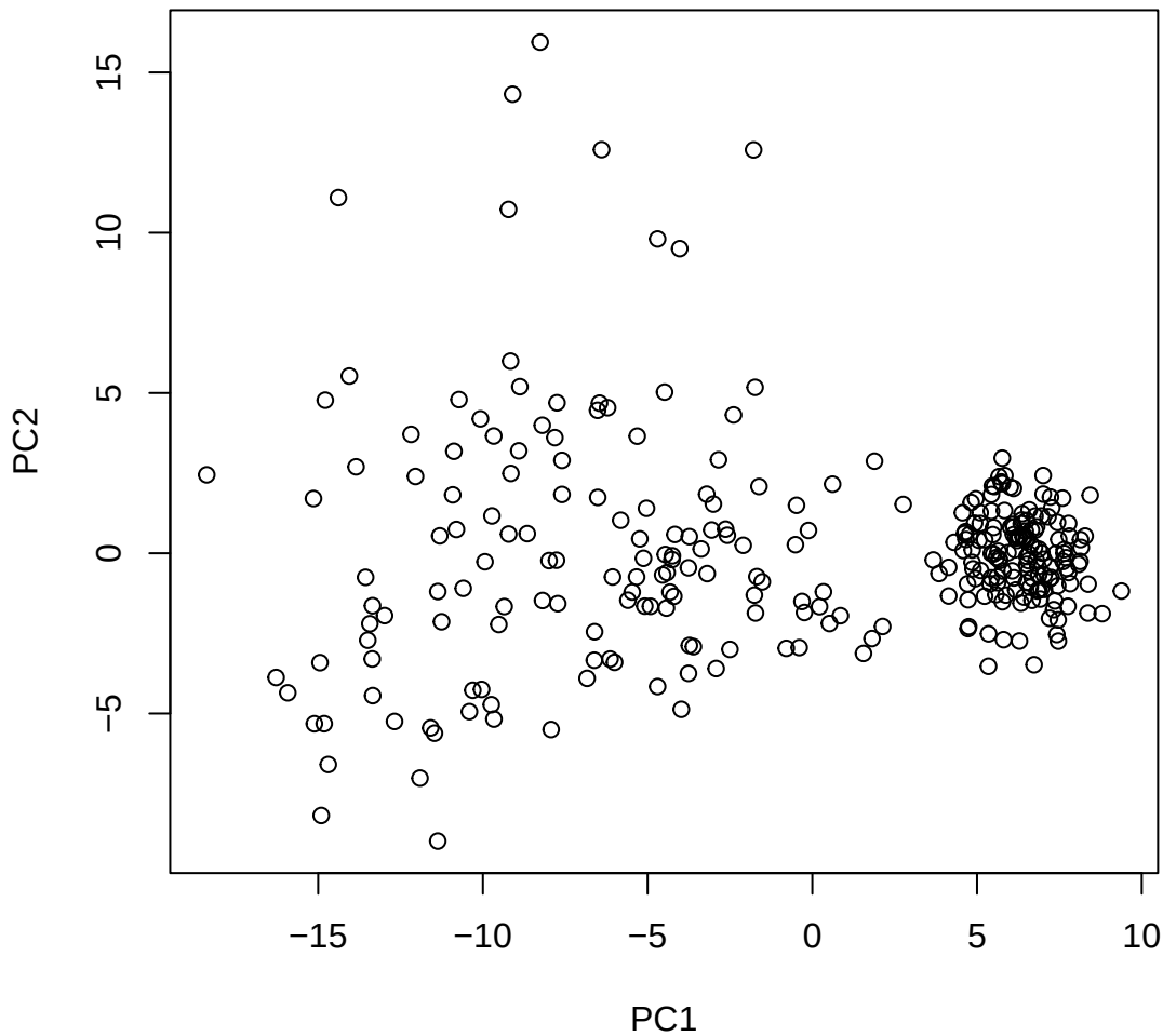
Window ID 134 NC_044062.1 (15)
