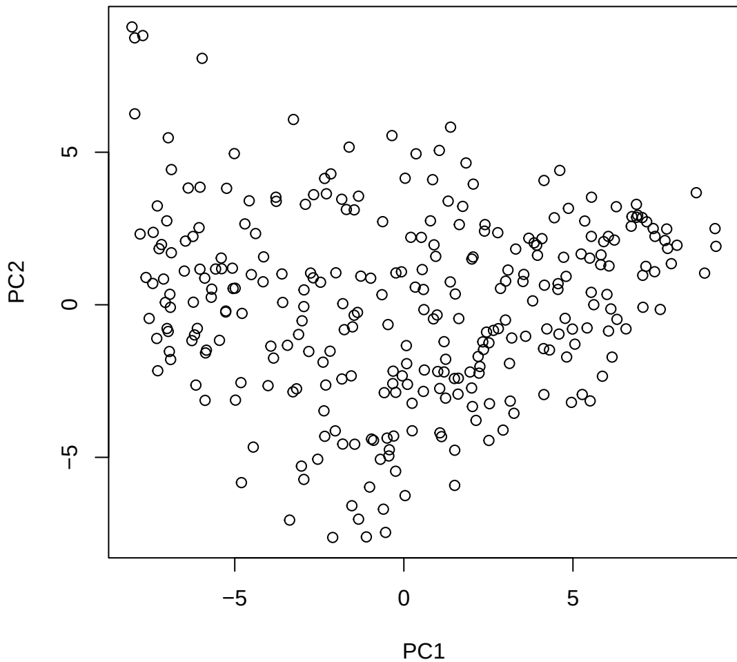
Window ID 139 NC_044062.1 (15)
