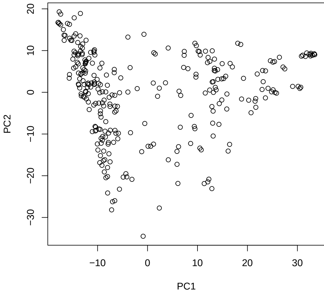
Window ID 145 NC_044063.1 (16)
