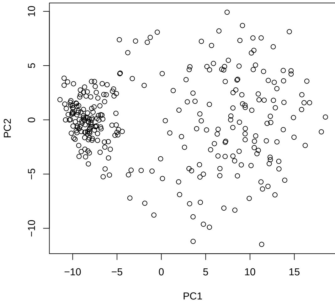
Window ID 156 NC_044065.1 (18)
