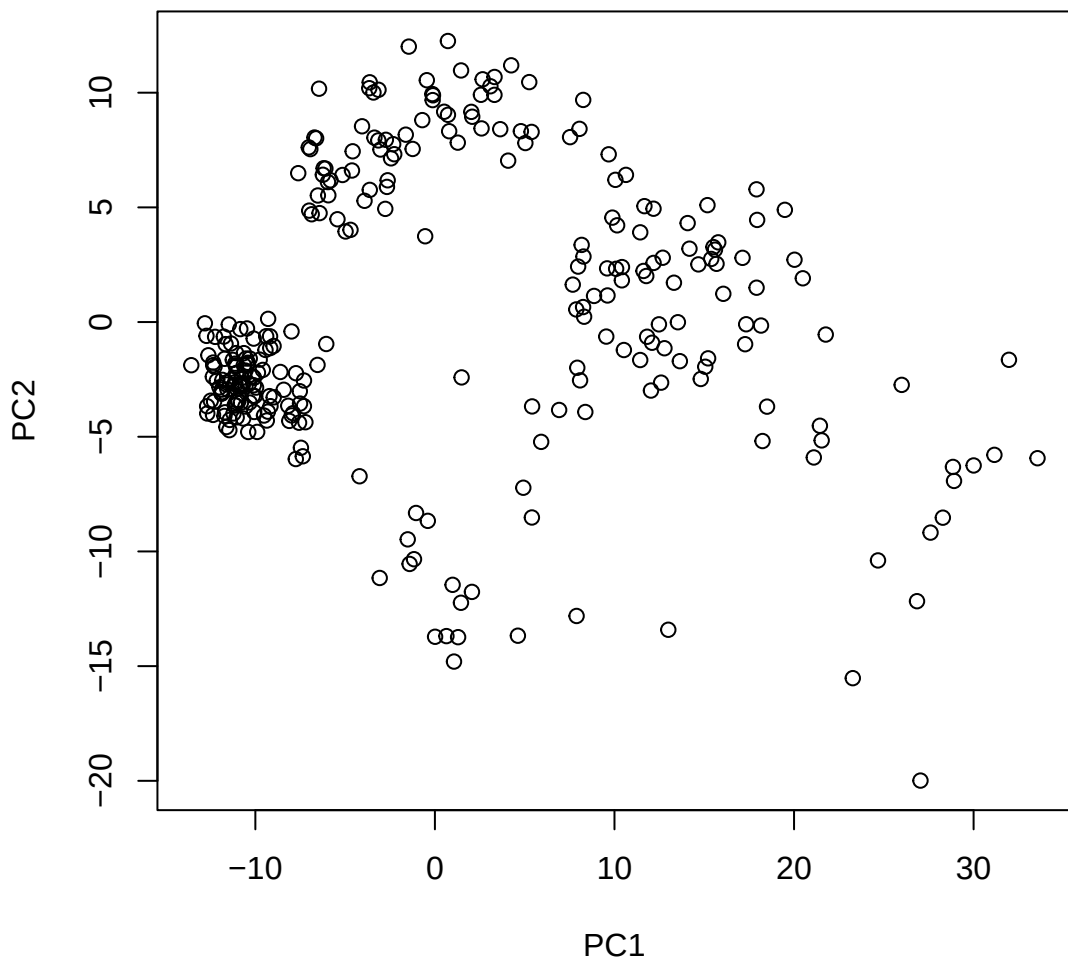
Window ID 163 NC_044065.1 (18)
