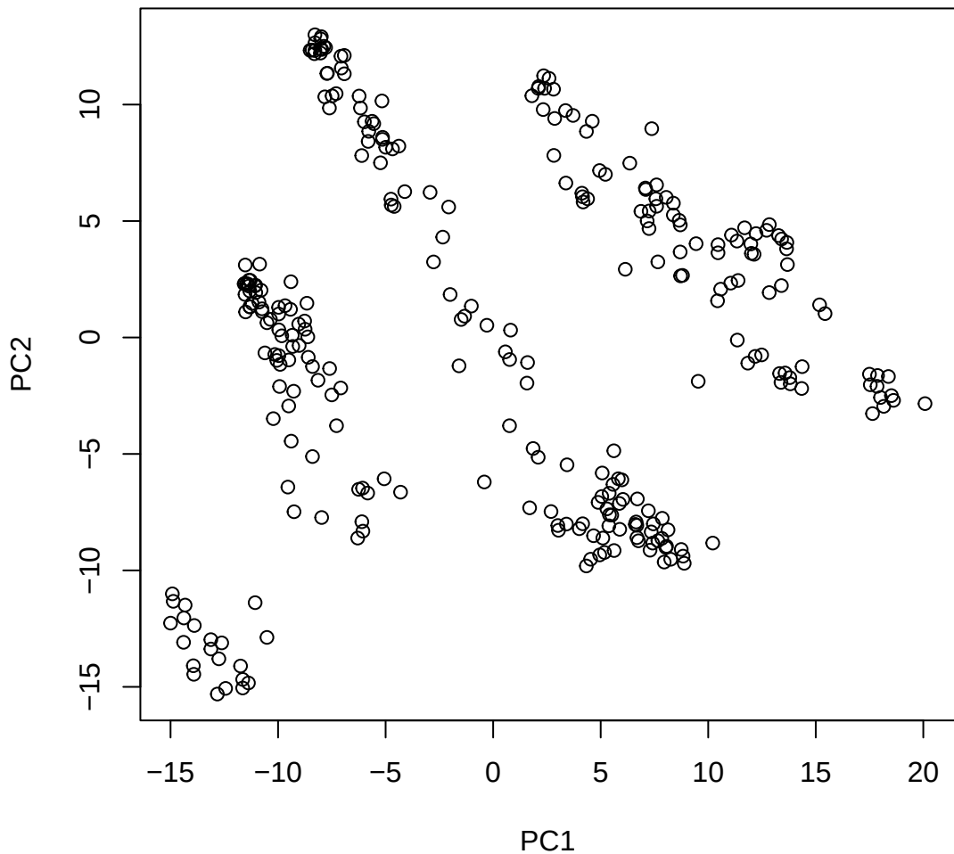
Window ID 177 NC_044067.1 (20)
