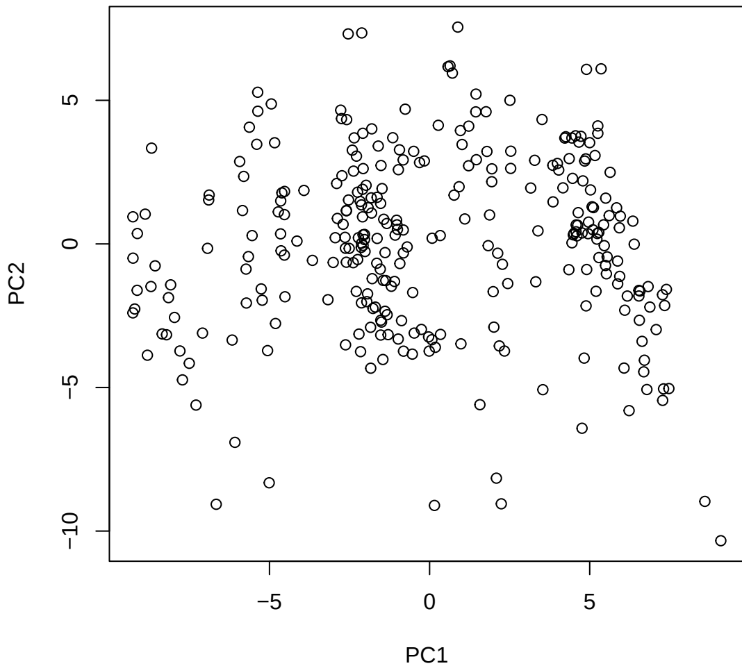
Window ID 187 NC_044068.1 (21)
