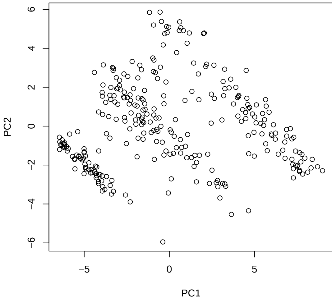
Window ID 14 NC_044048.1 (1)
