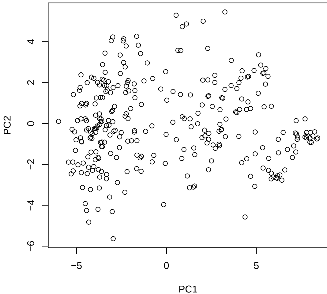
Window ID 15 NC_044048.1 (1)
