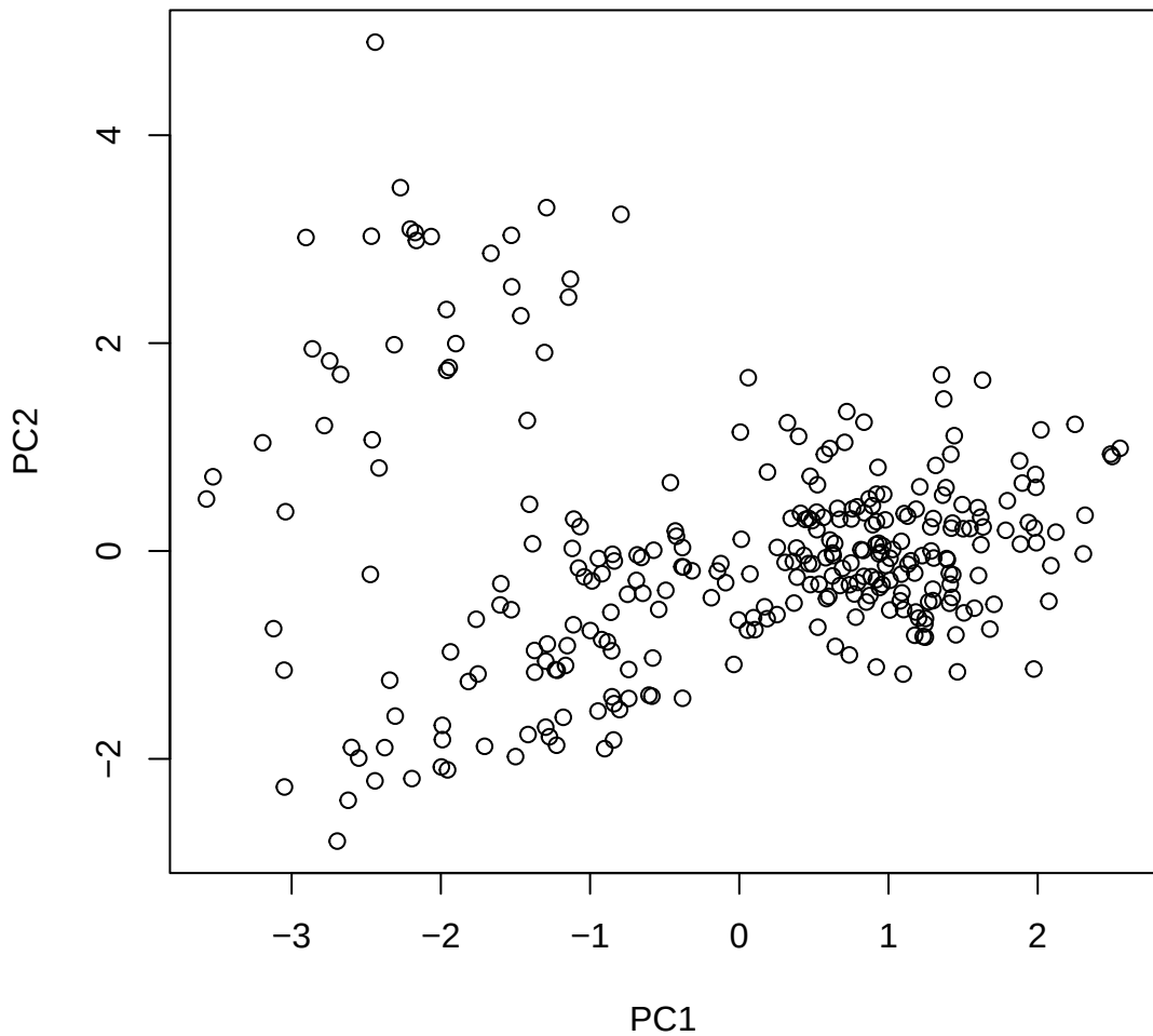
Window ID 24 NC_044048.1 (1)
