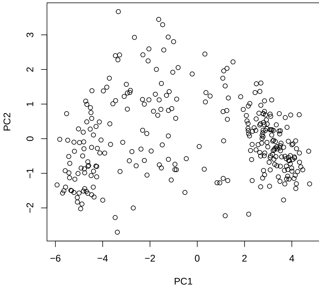
Window ID 77 NC_044050.1 (3)
