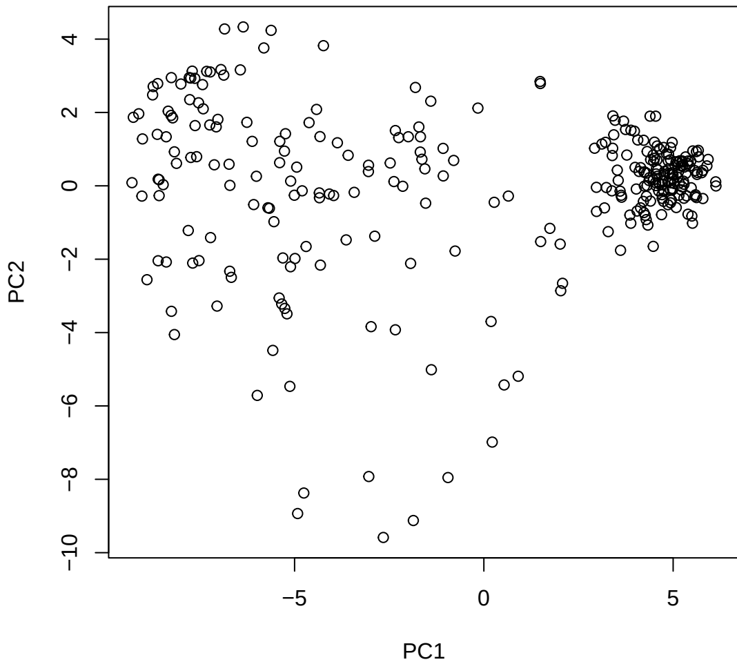
Window ID 111 NC_044051.1 (4)
